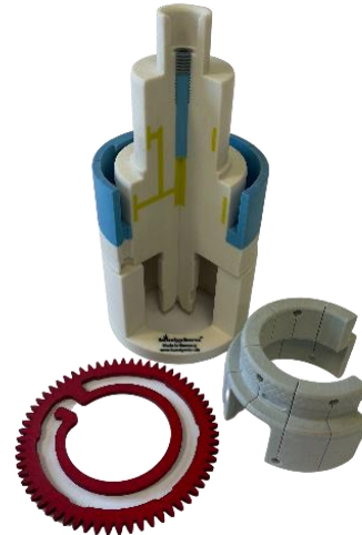
Illustration 3: Intermediate bushing and workpiece disassembled
